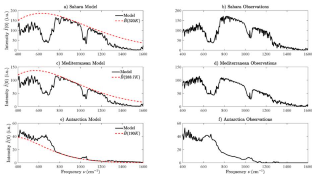
Figure 3. Modelled (left) and observed (right, from Nimbus satellite 1970) retention of radiative energy by \text{CO}_2 at typical regions like Sahara (upper), Mediterranean (middle) Antarctica (lower). The red, dotted lines are emissions from earth according to Planck distribution at the given temperatures. The area between the two lines represents the detained energy. From W. Weijngaarden and W. Happer 2020.
