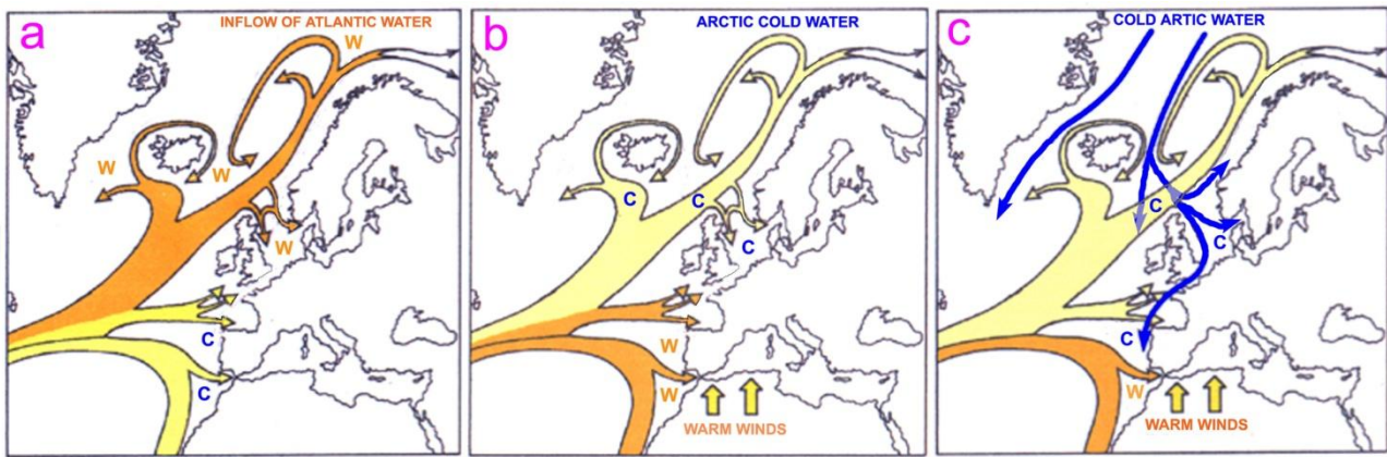
The beat of the Gulf Stream as a function of the Earth's rate of Rotation [3], [4], [5], [8]. Panel a) corresponds to Earth's deceleration during solar maxima. Panels b) and c) to Earth's acceleration during solar minima, with c) in deep solar minima like the Maunder 1687-1703 and Dalton 1808-1821 and maybe the next deep minimum.
