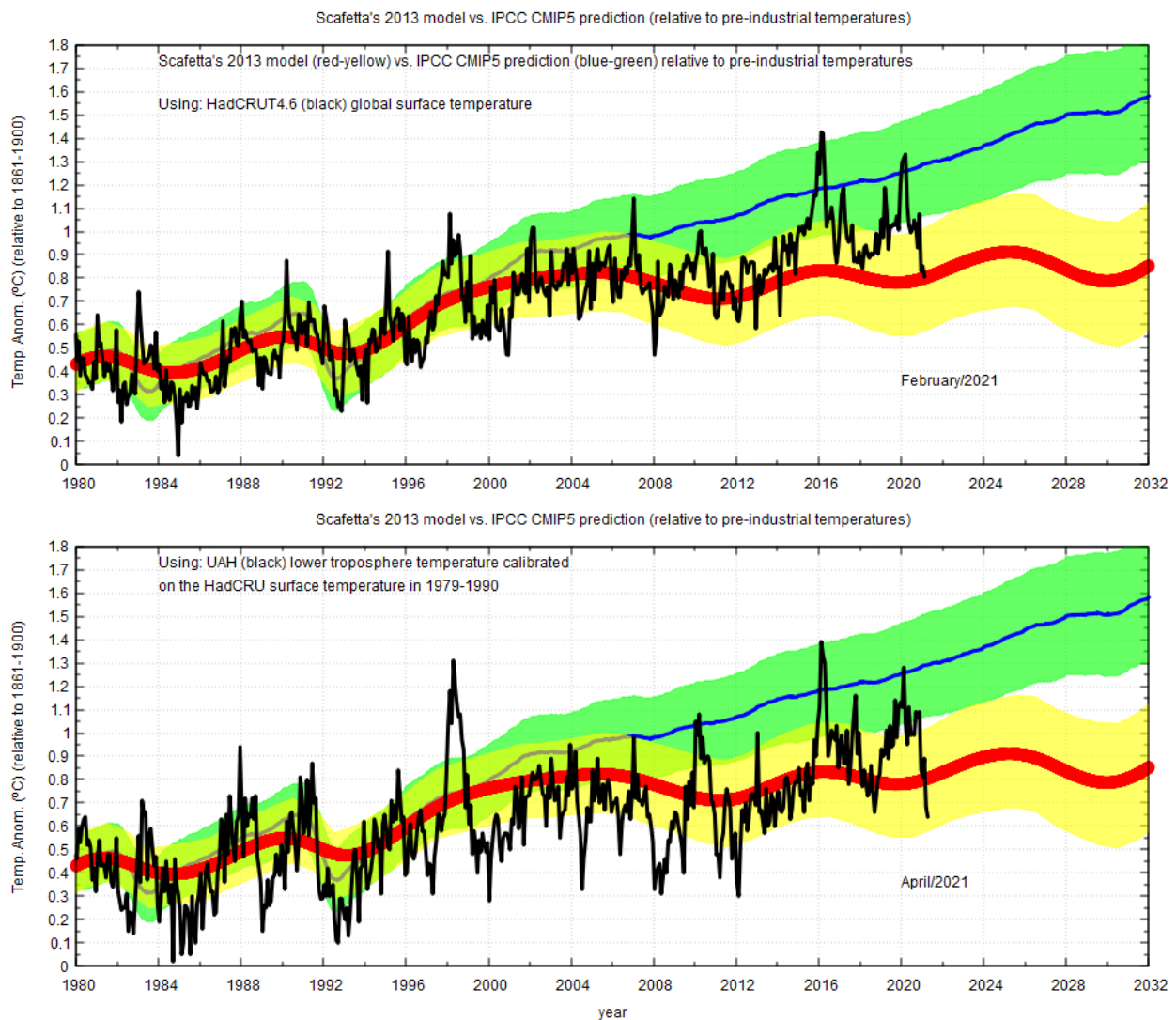
Figure 7. [Top] Zoom of Figure 6 bottom. [Below] The same model against the UAH lower troposphere global temperature record calibrated on the HadCRUT4.6 in the period 1979-1990. The green area indicates the prediction of the average CMIP5 models. The yellow one is the prediction of the model proposed in Scafetta (2013).
