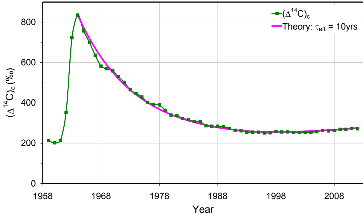
Figure 5: Evolution of calculated (\Delta^{14}\text{C})_c with effective absorption time of \tau_{\text{eff}} = 10 years (Magenta), compared against observed (\Delta^{14}\text{C})_c (Green).
